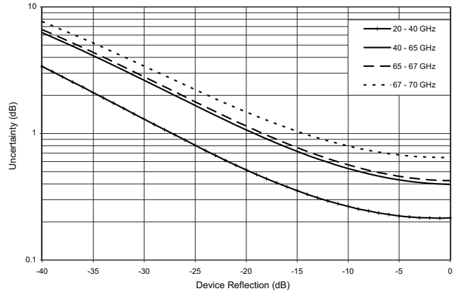
Reflection Magnitude Uncertainty (2 of 2) MS4647B with a 12-term Calibration using the 36585V AutoCal
