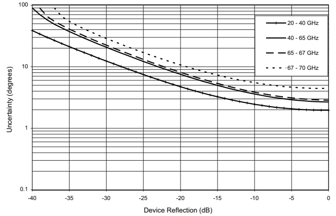
Reflection Phase Uncertainty (2 of 2) MS4647B with a 12-term Calibration using the 36585V AutoCal
