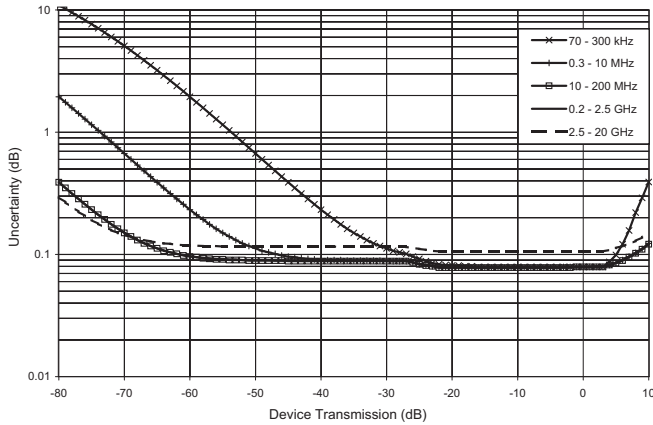
Transmission Magnitude Uncertainty (1 of 2) MS4647B with SOLT Calibration using 3654D Cal Kit
