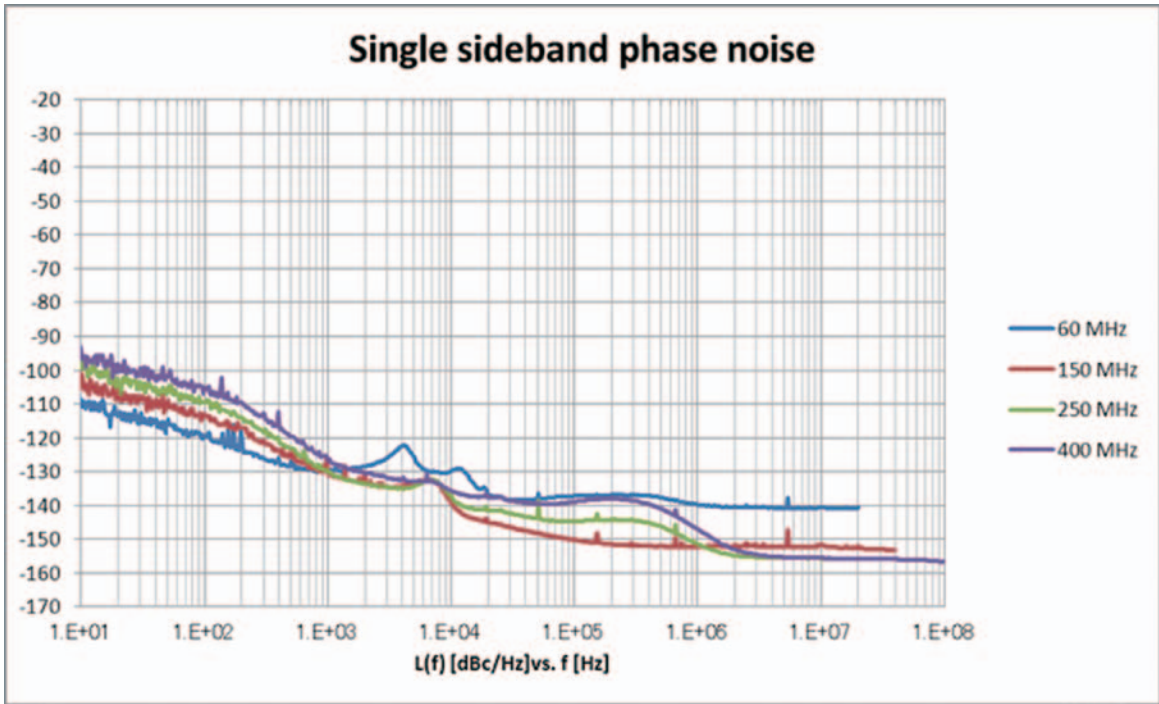
Phase Noise Optimization: <math>< 200\text{ kHz}</math>
