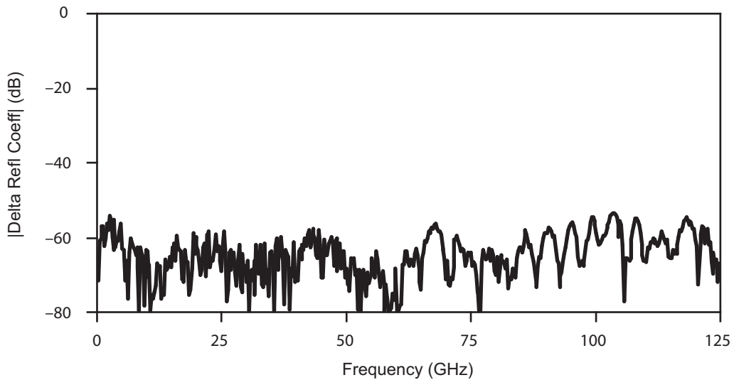
Example of vector delta thru line match after 24 hours
