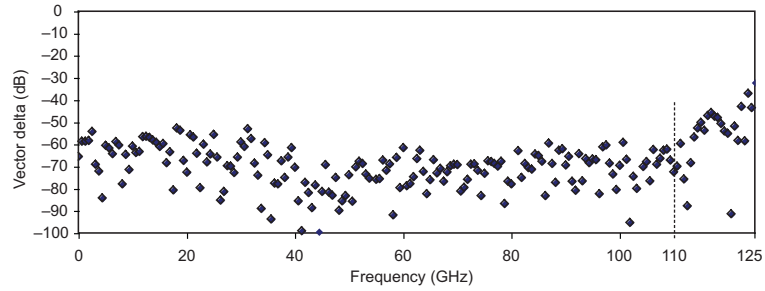
24 hour high reflect stability in vector delta format
