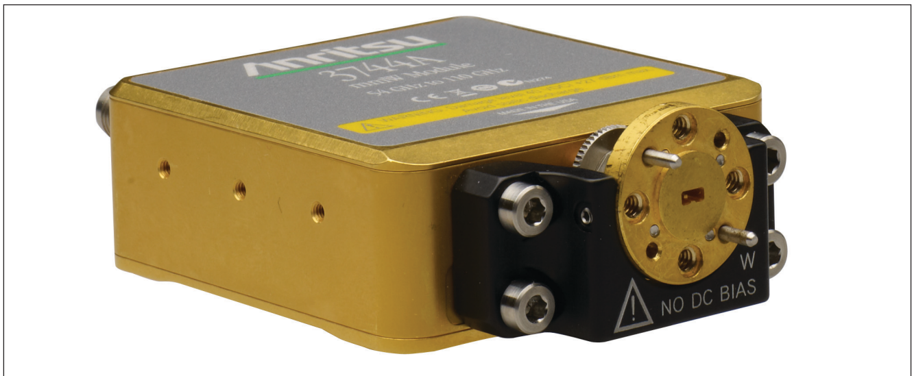
SM6499/SM6527 Millimeter-Wave Module with Waveguide Adapter
