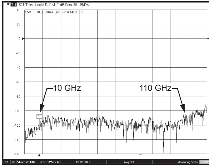
Dynamic range of ME7838A system at the W1 1 mm coaxial test port from 70 kHz to 125 GHz.
