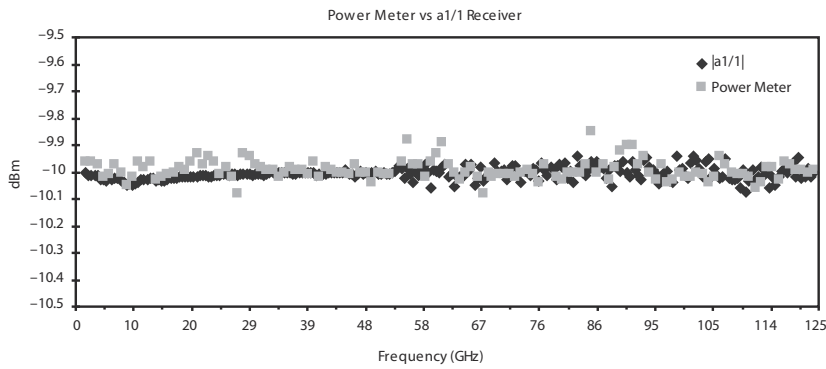
An example of power measurement agreement: power sensor vs. ME7838A a1 reference receiver.
