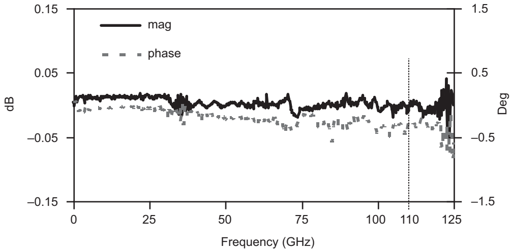
Thru line transmission stability up to 125 GHz
