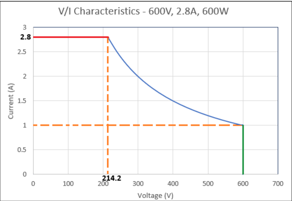
ASA Series 600W, 600V, 2.8A Voltage Vs Current Characteristics
