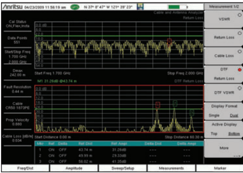
Dual Display
